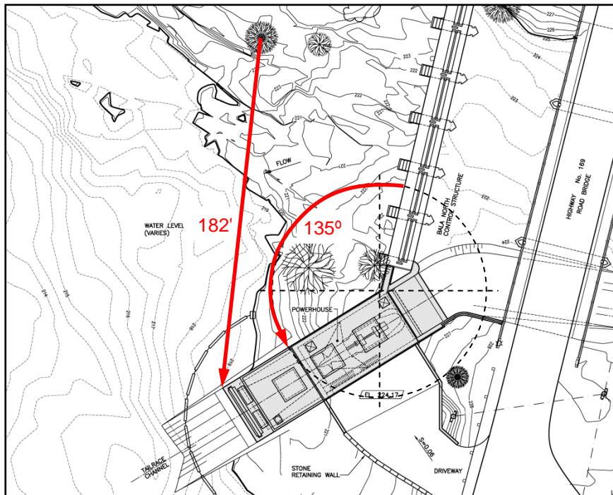
Cropped section of Alternative 1, General Arrangement (Option 1), from Page 2 of Appendix A of Environmental Screening Report
