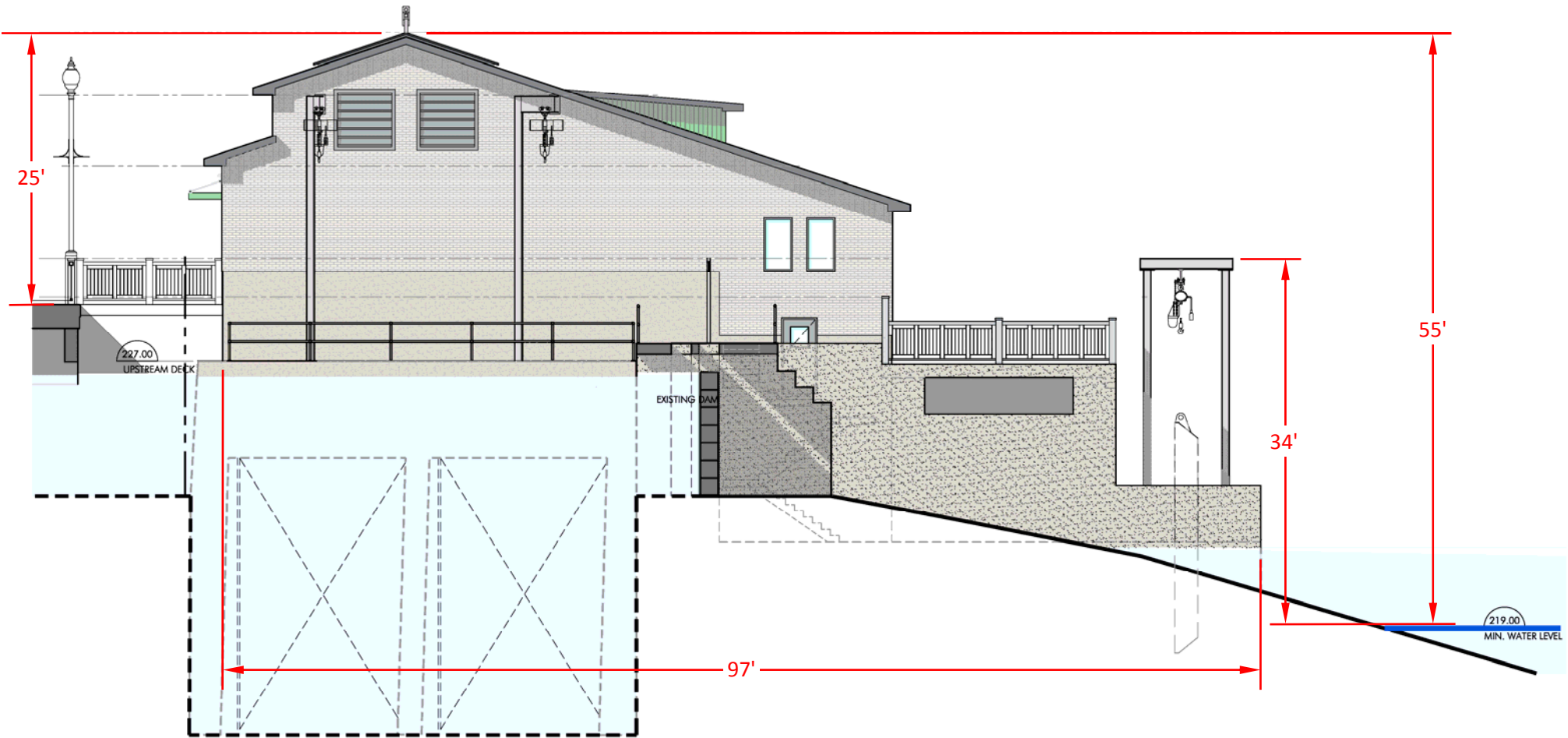
View looking south from Margaret Burgess Park of proposed hydro-electric generating station at the Bala falls.
