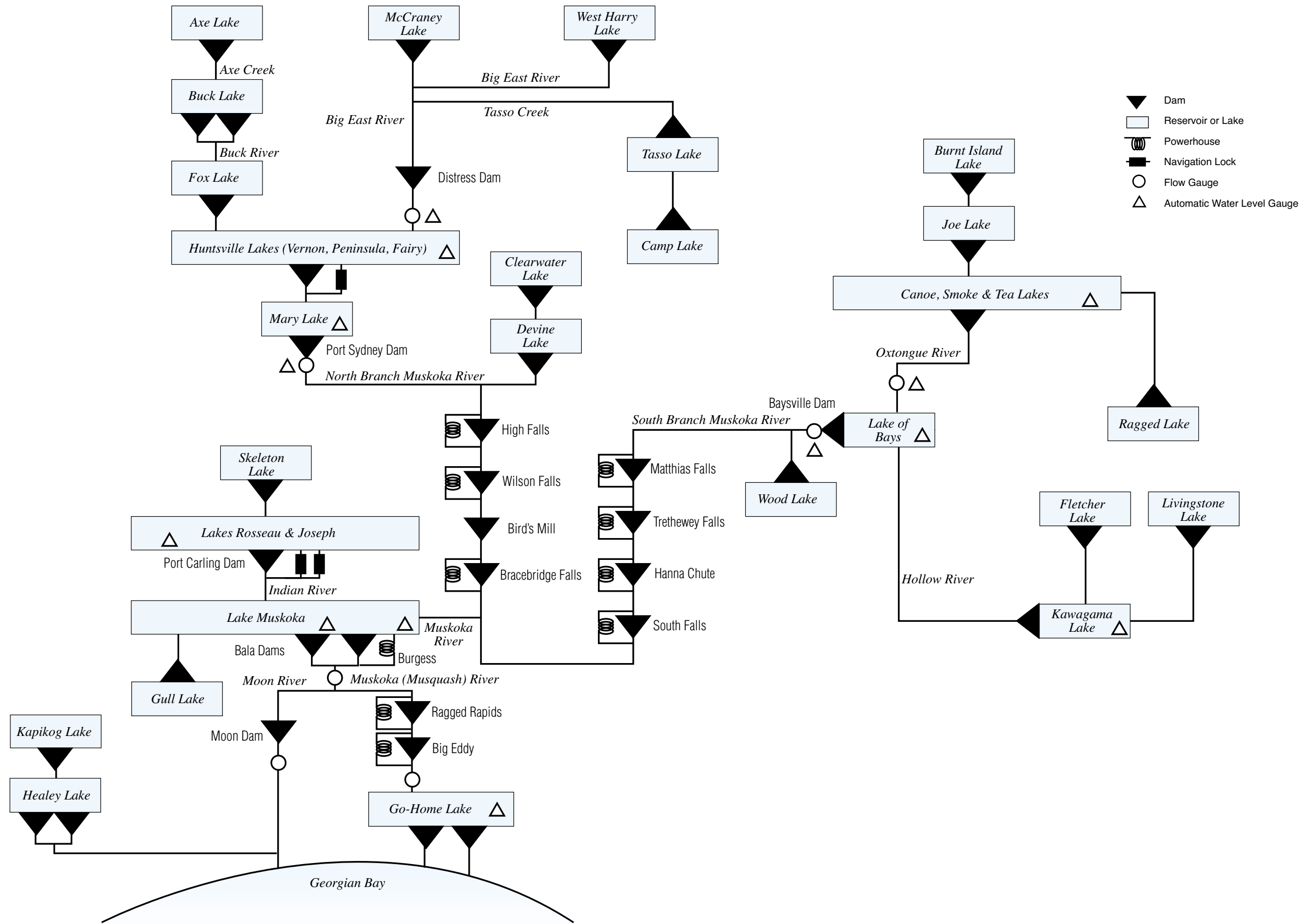
Figure 5.2 Muskoka River Water Management Plan Control Structure Schematic
